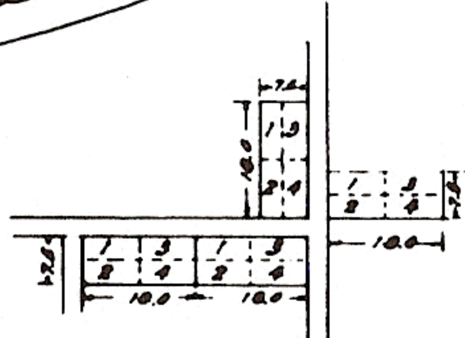
REGULAR GRAVE LAYOUT LOTS - 7.5 x 18.0 FT. GRAVES - 3.75 x 9.0 FT. WALKS - 3.0 FT.
